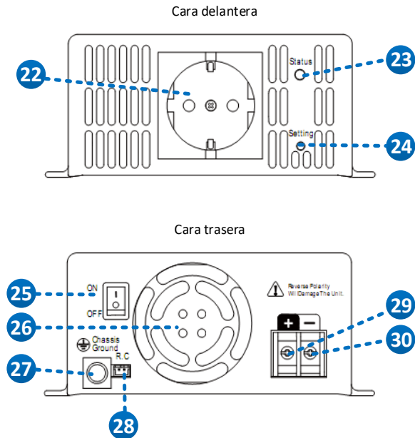
Fig. 5 Inversor monofásico TS-400/ Single phase inverter TS-400.
